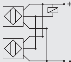
Parallel connection
