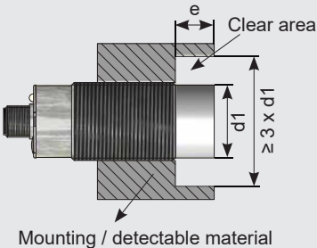
Non-flush mountable
