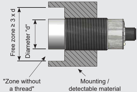
Fig. 2 Non-flush mountable
