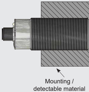
Fig. 1 Flush mountable
