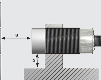
Fig. 4 Non-flush mountable
