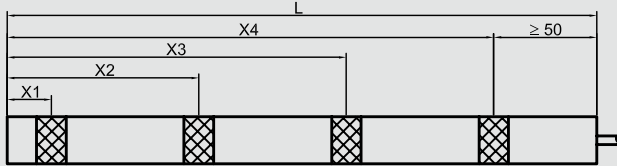
Fig. 3 KFS-4-.../KFX-4-... probe with variable limit value switching points
